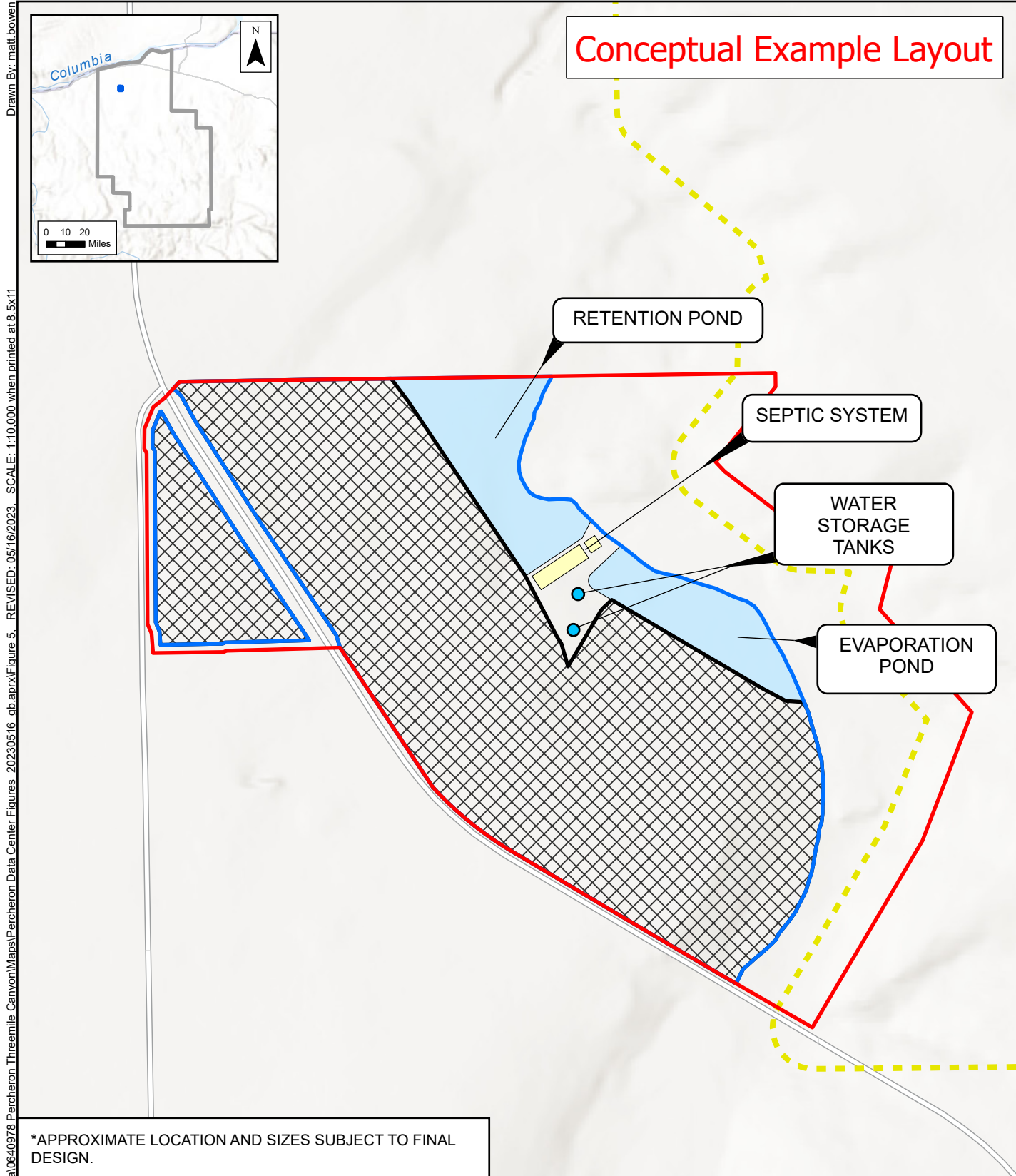
Figure 5 Preliminary Project Layout Percheron Data Center Rowan Percheron, LLC Morrow County, Oregon
