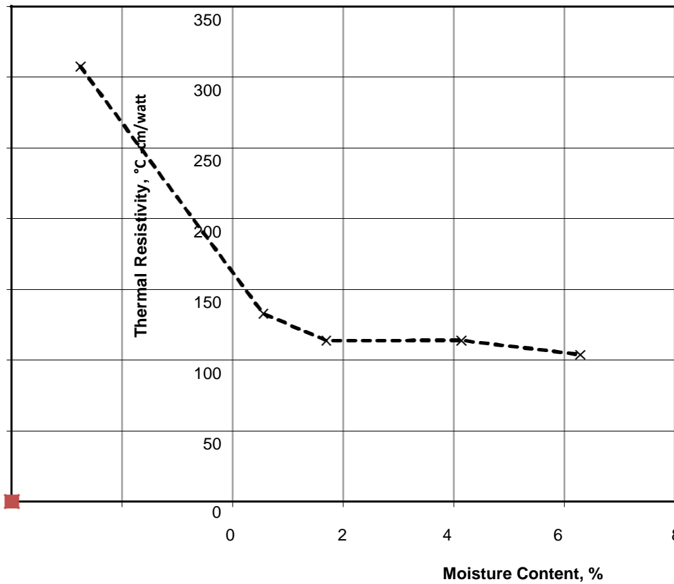
Thermal Resistivity Dry-Out Curve
