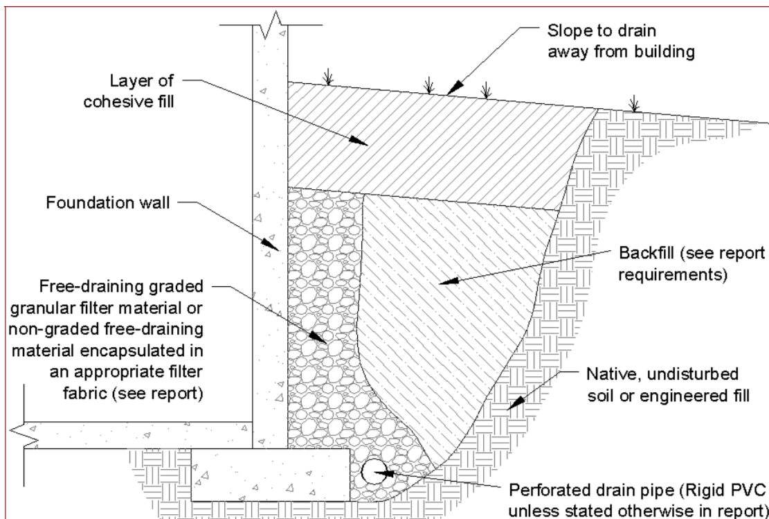
Diagram 4: Retaining Wall Backfill and Drain Placement
